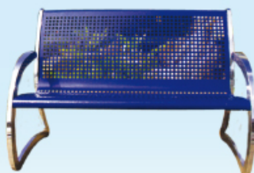
Model: BC-700EG/(DC) Dimension : 1250(L) x 665(W) x 910(H)mm Weight : 29 kg Model: BC-701EG/(DC) Dimension : 1550(L) x 665(W) x 910(H)mm Weight : 34.5 kg Model: BC-702EG/(DC) Dimension : 1850(L) x 665(W) x 910(H)mm Weight : 39.5 kg
