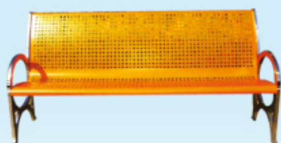
Model: BC-300EG/(DC) Dimension : 1250(L) x 665(W) x 910(H)mm Weight : 30 kg Model: BC-301EG/(DC) Dimension : 1550(L) x 665(W) x 910(H)mm Weight : 35 kg Model: BC-302EG/(DC) Dimension : 1850(L) x 665(W) x 910(H)mm Weight : 40.5 kg
