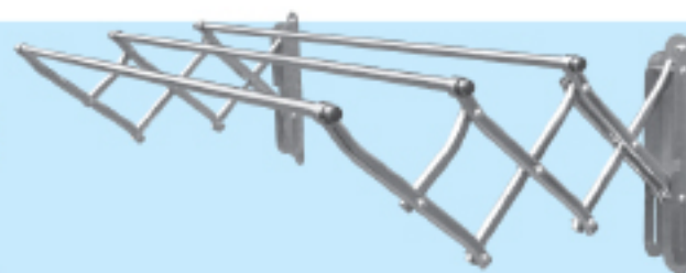
Stainless Steel Retractable Rack Model: SRR 300/(DC) Size: 914(L) x 508(W) x 316(H)mm Model: SRR 400/(DC) Size: 1219(L) x 747(W) x 416(H)mm Model: SRR 500/(DC) Size: 1524(L) x 994(W) x 516(H)mm
