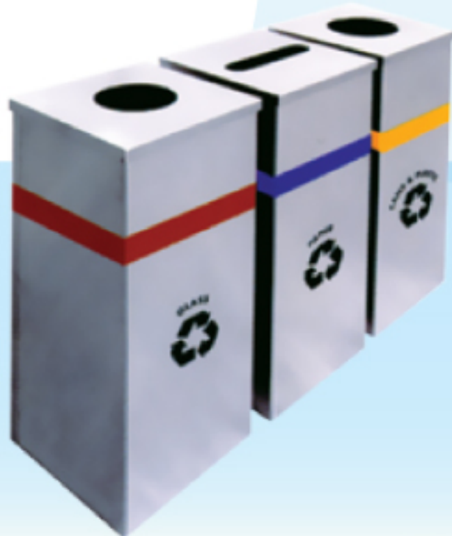
Stainless Steel Square Recycle Bin Model:SARB-010/(DC) Size: 300(L) x 300(W) x 740(H)mm
